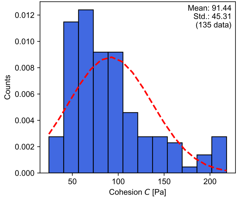
Reactivation cohesion C_R
