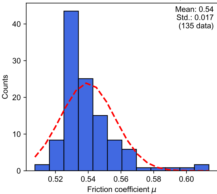
Reactivation friction coefficient \mu_R
