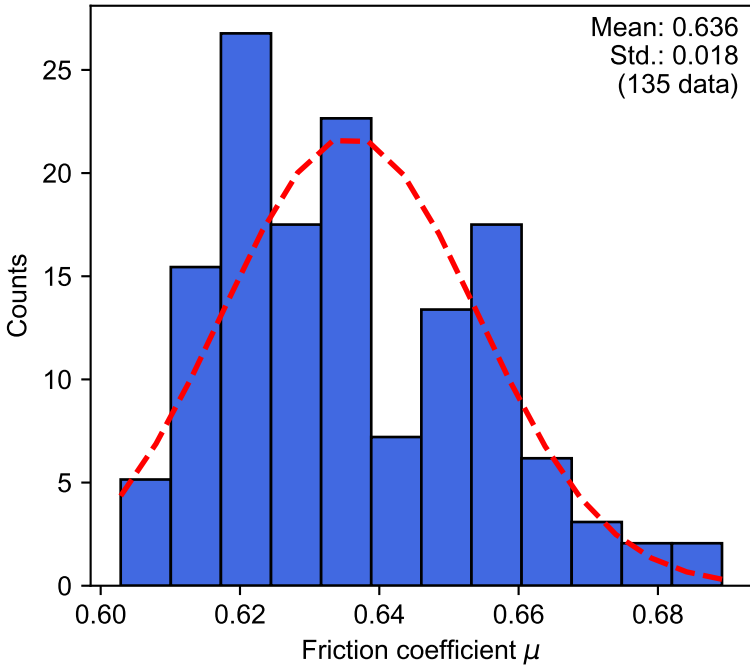
Dynamic friction coefficient \mu_D
