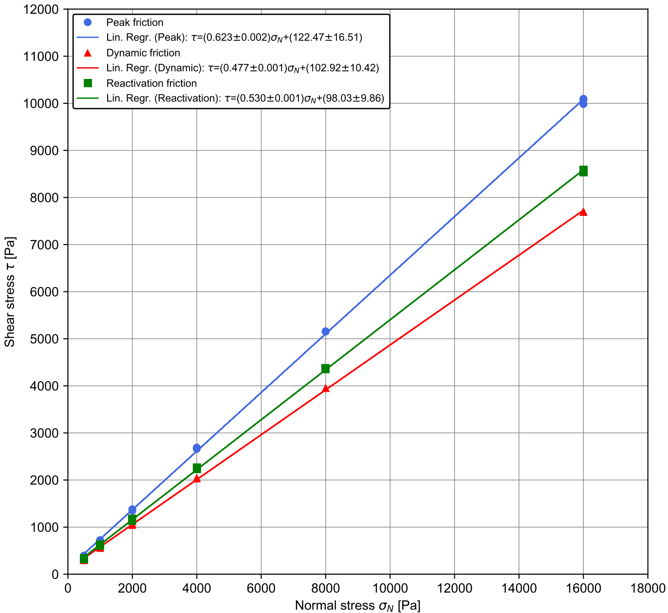
378-01_CDUT-L2 (18 measurements)
