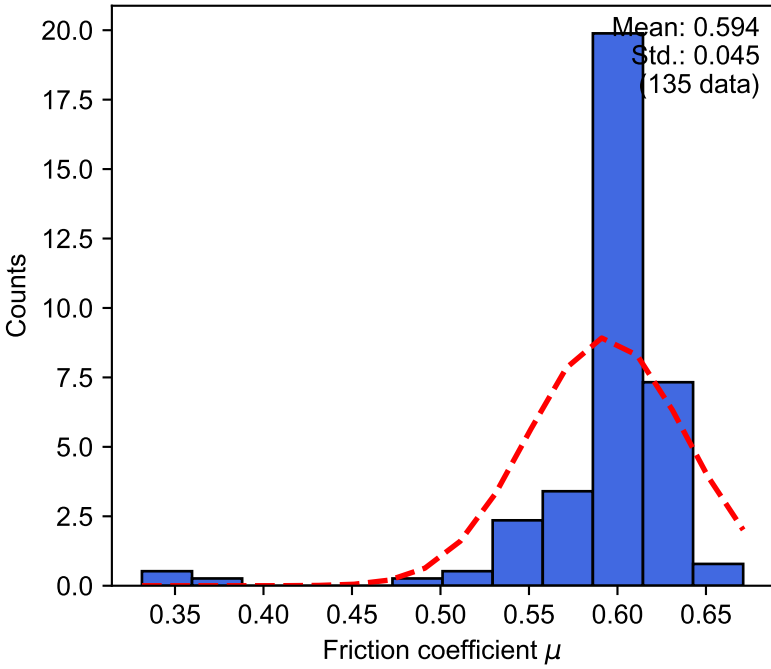
Dynamic friction coefficient \mu_D
