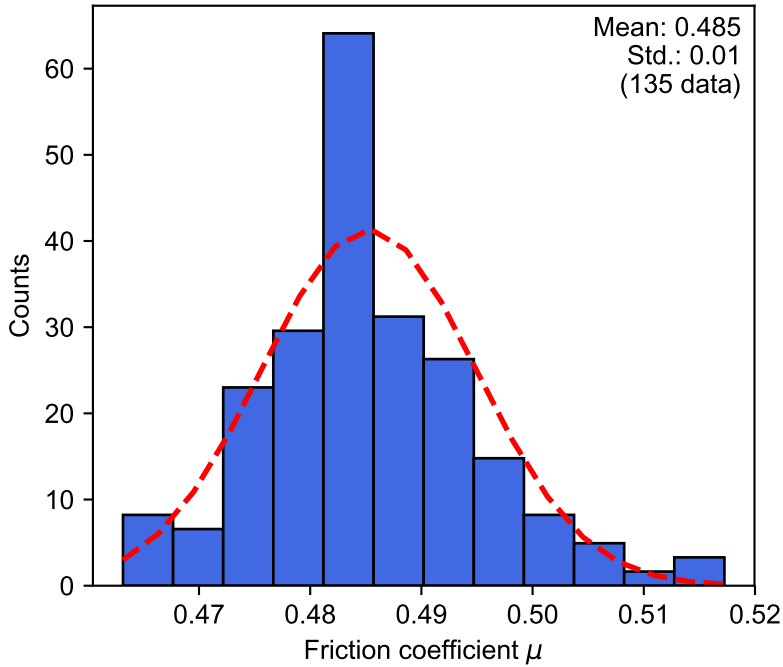
Reactivation friction coefficient \mu_R
