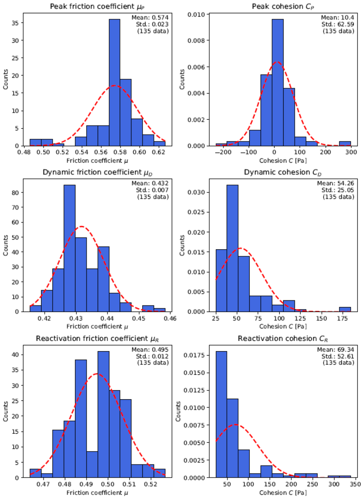
Figure 4: Example of histogram plot (437-01). Histograms of mutual two-point regression results for slope (friction coefficient \mu ) and y-axis intercept (cohesion C). Red curves are synthetic normal distributions with the same mean and standard deviation (std.) as the data set for comparison ( v = \text{shear velocity} = 30 \text{ mm min}^{-1} ).
