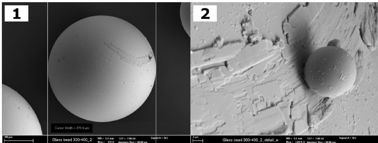
Figure 1: Examples of microscopic images of the tested materials. (1) single glass bead 300-400 \mu\text{m} at 175x magnification, (2) surface of a glass bead at 3000x magnification with a smaller glass bead on it.
