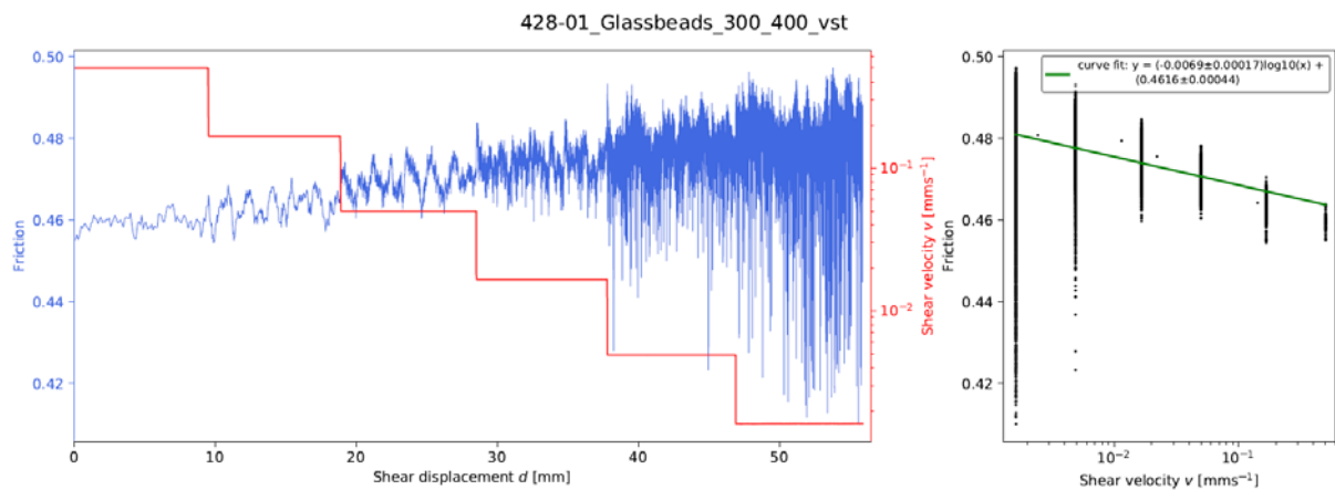
Figure 5: Example of the visualization of the VST data (428-01). The shear velocity v is decreased stepwise (red curve), while the dynamic friction (shear stress \tau /normal stress \sigma N ) is measured (blue curve). The logarithmic fit (green curve) reflects the slight decrease of the friction with increasing shear velocity v .
