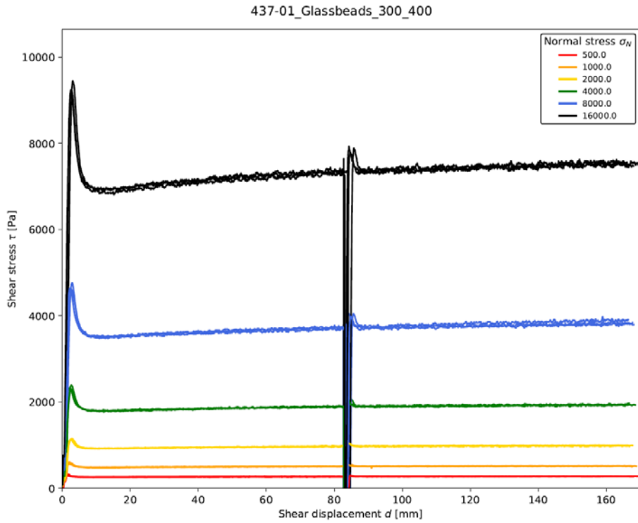
Figure 2: Example of shear curve plot (437-01). Y-axis is shear stress \tau , x-axis is shear displacement d . Each data set consists of 18 shear curves corresponding to 6 levels of normal stress \sigma_N with 3 repetitions each stress level ( v = \text{shear velocity} = 30 \text{ mm min}^{-1} ).
