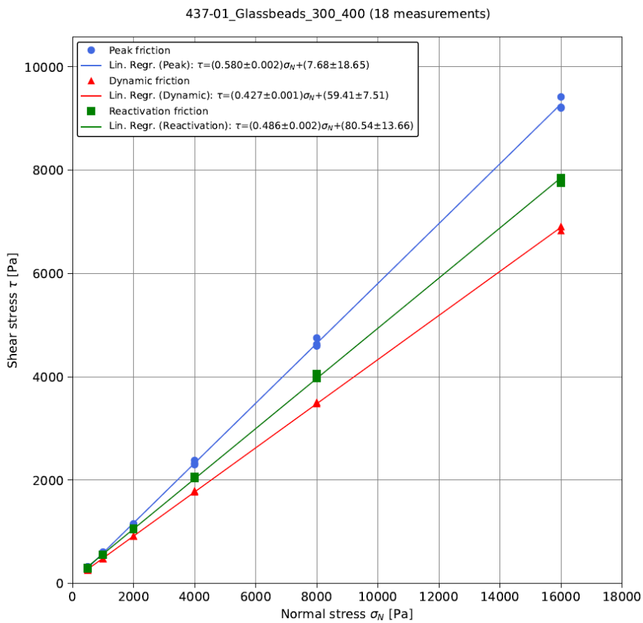
Figure 3: Example of friction plot (437-01). Plot of all data pairs in the Mohr space (normal stress \sigma_N vs. shear stress \tau ) including curves of the corresponding linear least-squares ( v = \text{shear velocity} = 30 \text{ mm min}^{-1} ).
